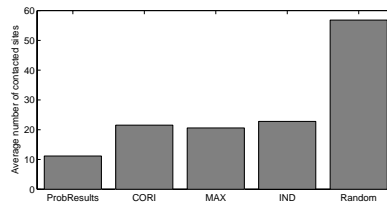
Fig. 9. Comparison of ranking functions - dynamic scenario.
