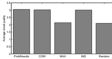
Fig. 8. Quality comparison of ranking functions - static scenario.
